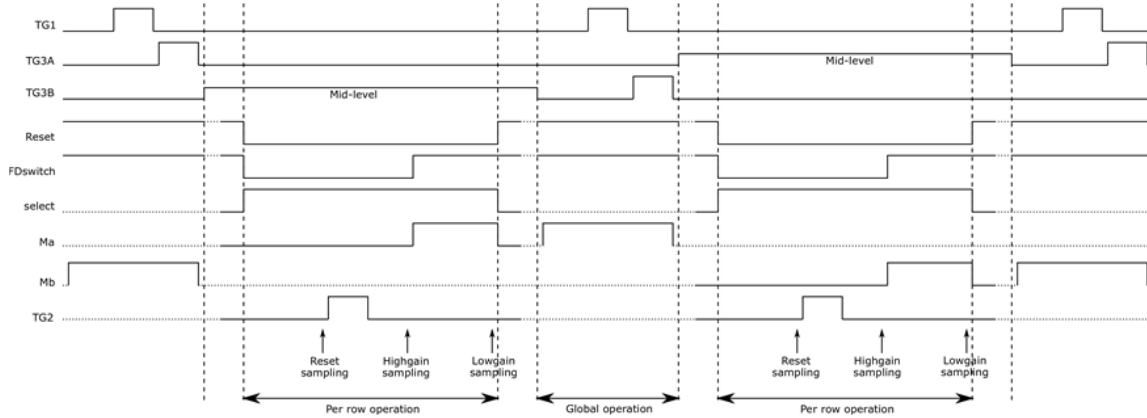
Figure 10: Typical global shutter timing
