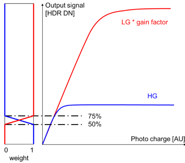
Figure 7: Weighted interpolation between HG and LG signals
