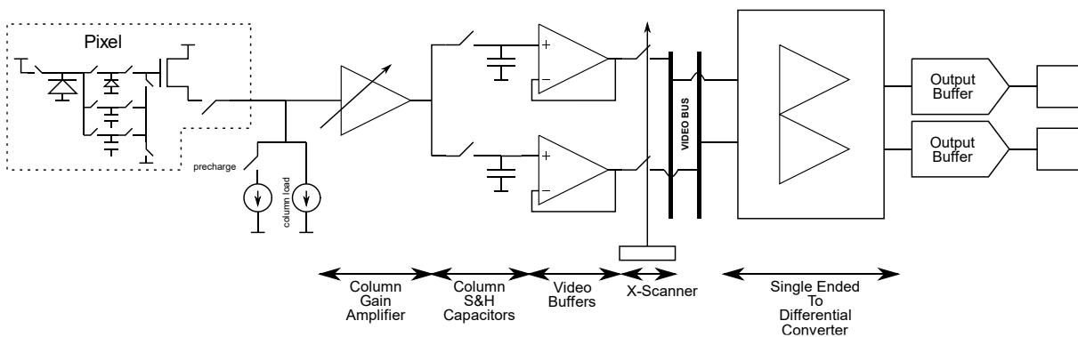
Figure 9: Simplified analog chain
