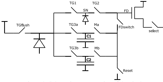
Figure 2: Schematic representation of the pixel
