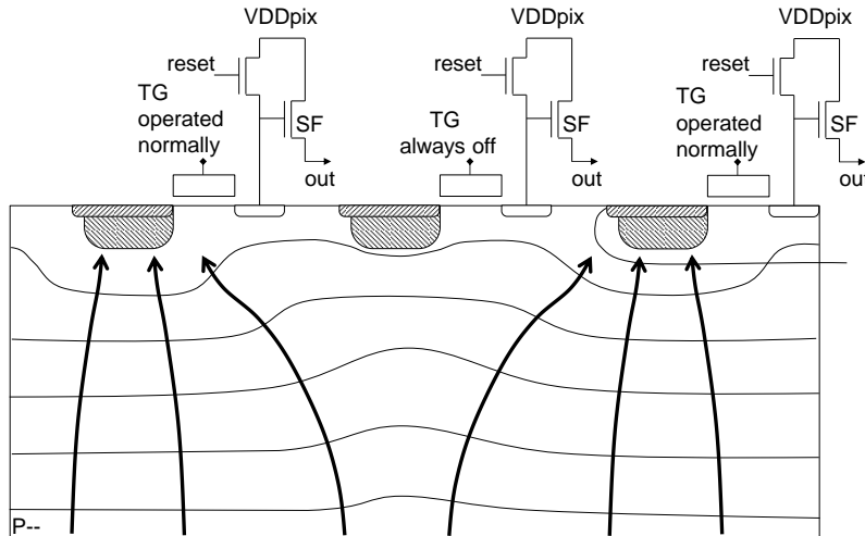
Figure 8: cross sections of three pixels, showing the ELFIS2 concept of charge domain binning.
